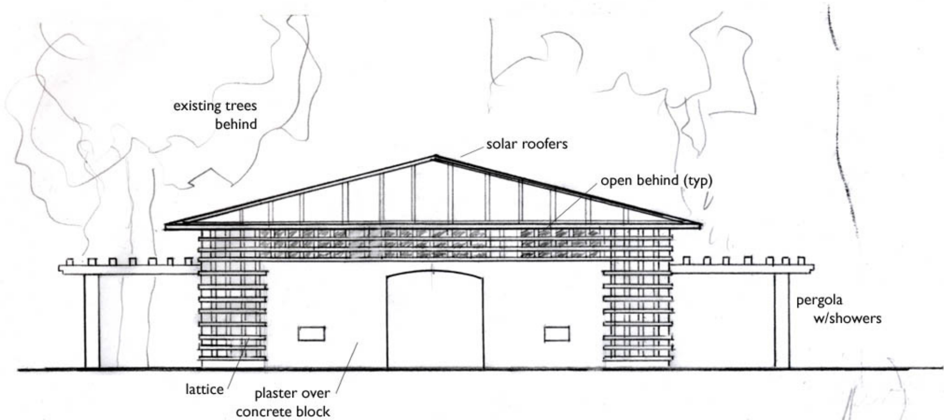
East Elevation
